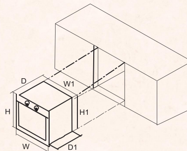
BUILT-IN MICROWAVE OVENS
